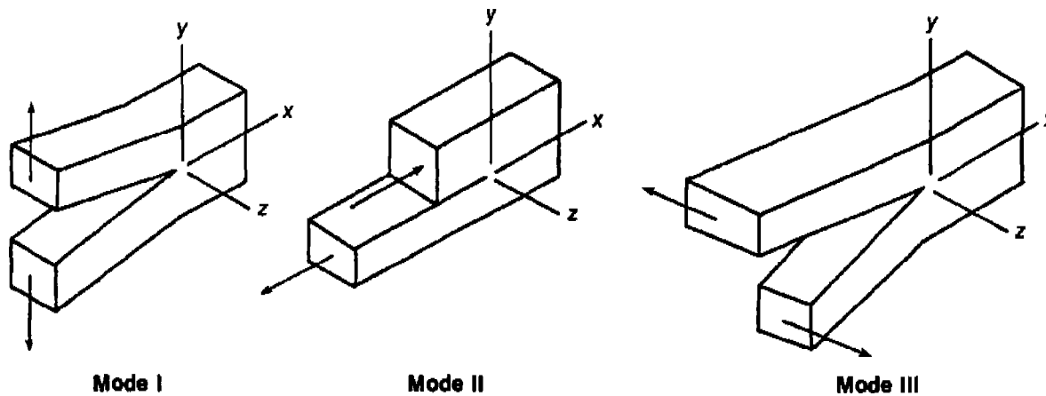
Figure 4-10 Basic Modes of Loading Involving Different Crack Surface Displacements [ASM, Engineered Materials Handbook ]
