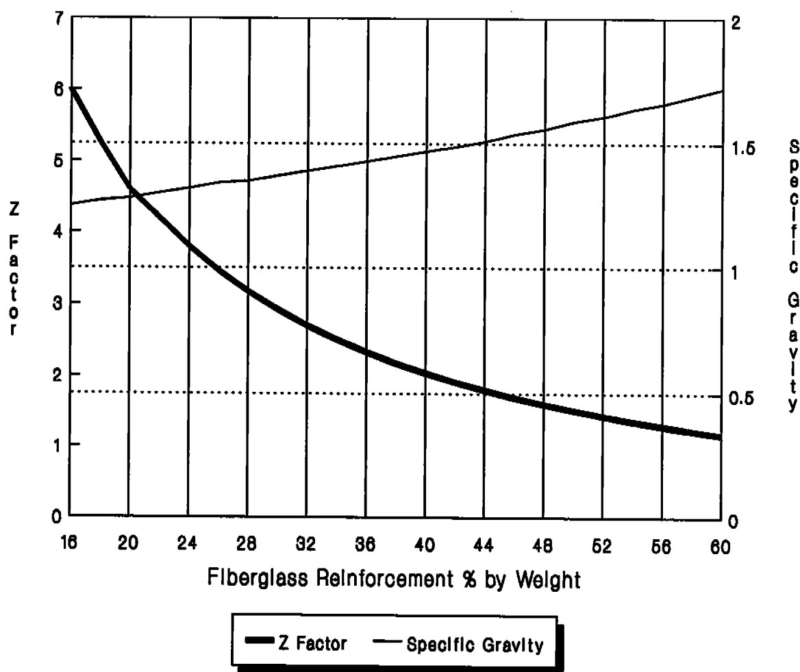
Figure 3-21 Z-Factor and Approximate Laminate Specific Gravity for Fiberglass Laminates with Unfilled Resin Systems [Owens-Corning Fiberglas, The Hand Lay-Up and Spray-Up Guide ]
