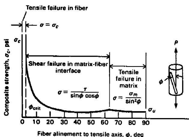
Figure 3-14 Failure Mode as a Function of Fiber Alignment [ ASM Engineers' Guide to Composite Materials ]
