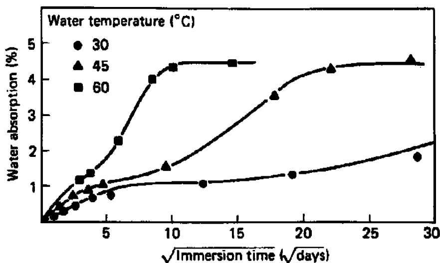
Figure 4-15 Laminate Water Absorption Kinetics for Experimental Laminate Specimens [Pritchard, The Use of Water Absorption Kinetic Data to Predict Laminate Property Changes ]
