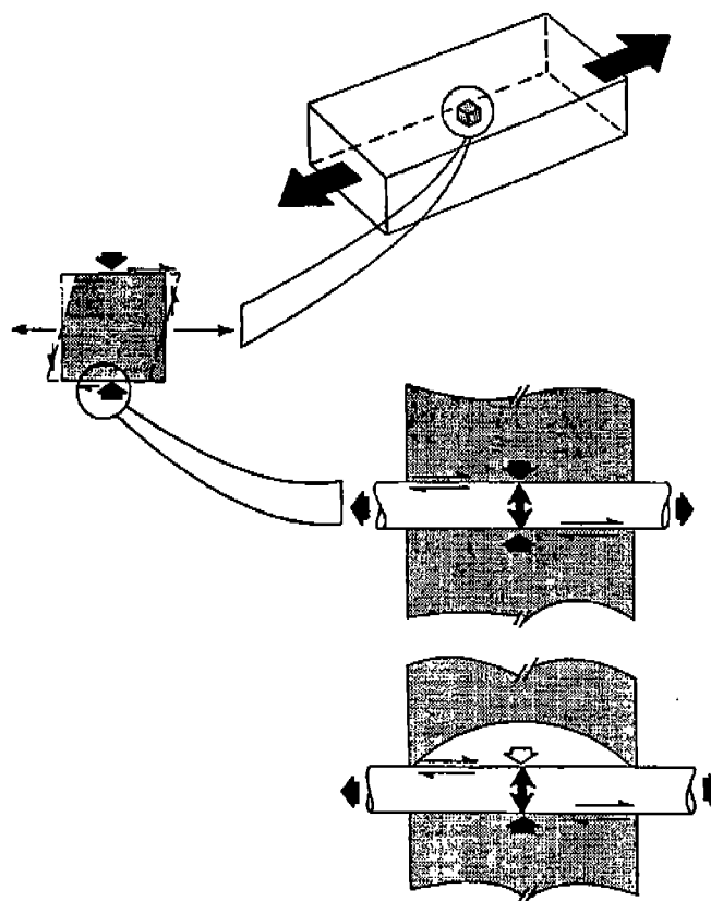
Figure 3-13 State of Stress and Stress Transfer to Reinforcement [ Material Engineering , May, 1978 p. 29]
