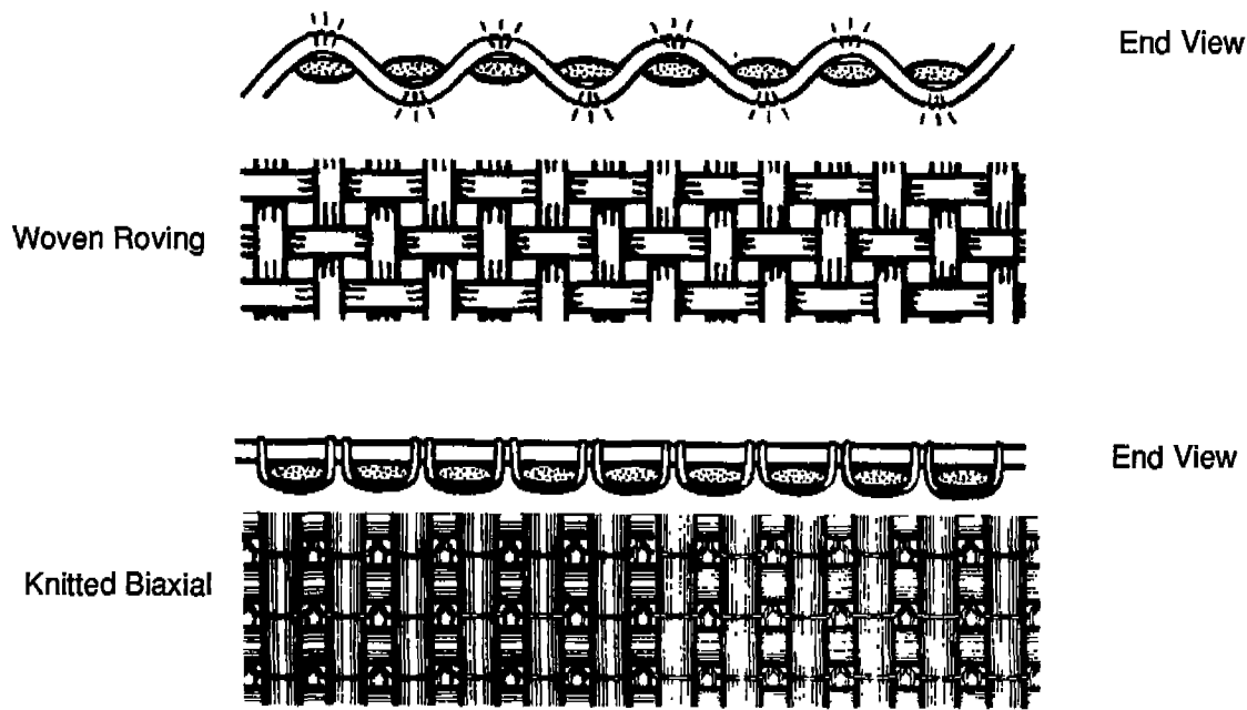
Figure 2-4 Comparison of Conventional Woven Roving and a Knitted Biaxial Fabric Showing Theoretical Kink Stress in Woven Roving [Composites Reinforcements, Inc.]
