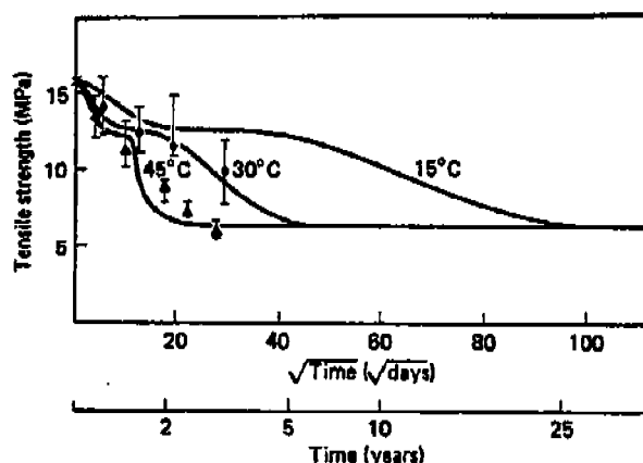
Figure 4-17 Predicted Wet Tensile Strength versus Square Root of Immersion Time [Pritchard, The Use of Water Absorbition Kinetic Data to Predict Laminate Property Changes ]
