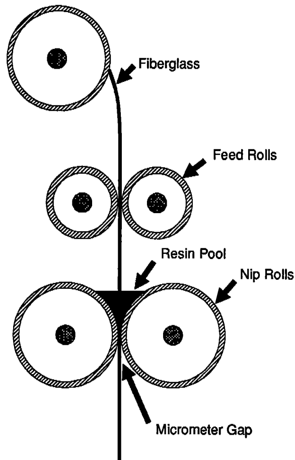
Figure 5-12 Impregnator Material Path [Raymer, Large Scale Processing Machinery for Fabrication of Composite Hulls and Super-structures ]
