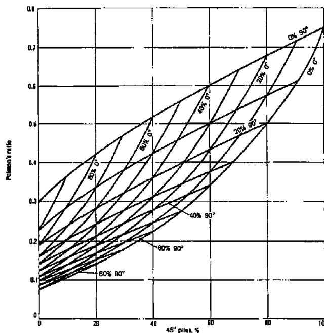
Figure 3-20 Carpet Plot Illustrating Poisson's Ratio [ASM Engineered Materials Handbook]
