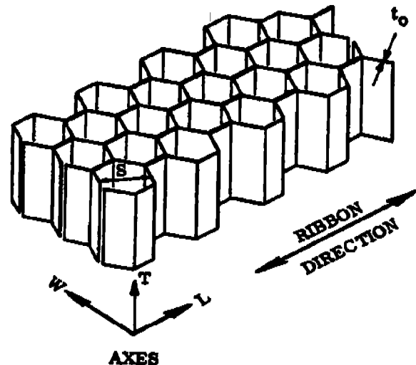
Figure 2-8 Hexagonal Honeycomb Geometry [MIL-STD-401B]
