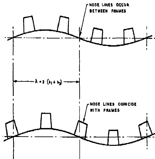
Figure 3-10 Extraframe Buckling Modes [Smith, Buckling Problems in the Design of Fiberglass-Reinforced Plastic Ships ]
