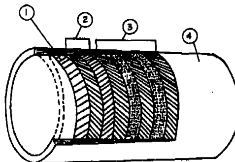
Figure 1-11 Cutaway View of Contact-Molded Pipe [Cheremisinoff, Fiberglass-Reinforced Plastics Deskbook ]
