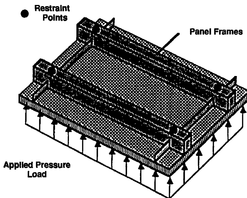
Figure 6-6 Schematic Diagram of Panel Testing Pressure Table [Reichard]
