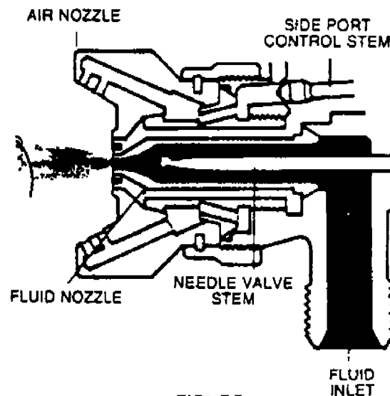
Figure 5-8 Airless Spray Gun Showing Possible Bounce Back from the Mold [Venus-Gusmer]
