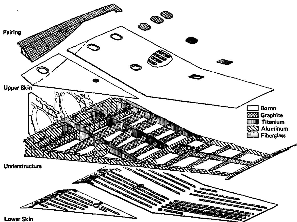
Figure 1-15 Composite Wing Composition for Advanced Tactical Fighter [Moors, Design Considerations - Composite Flight Wing Program ]
