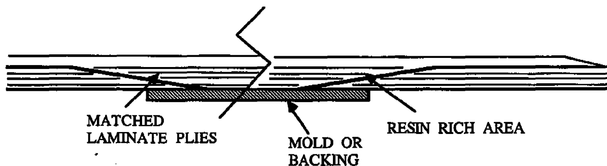
a) Conventional Taper Sequence for FRP Repairs
