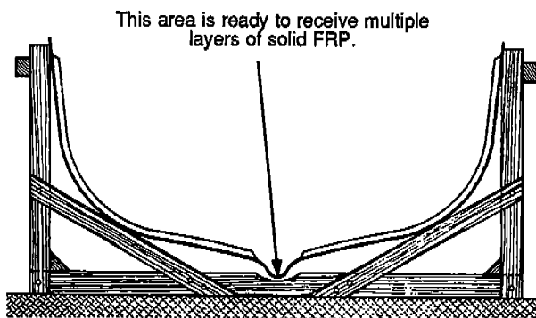
Receiving Mold with Hull Consisting Of Core and Outside Skin.
