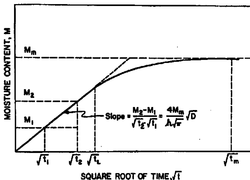
Figure 4-14 Change of Moisture Content with the Square Root of Time for "Fickian" Diffusion [Springer, Environmental Effects on Composite Materials ]
