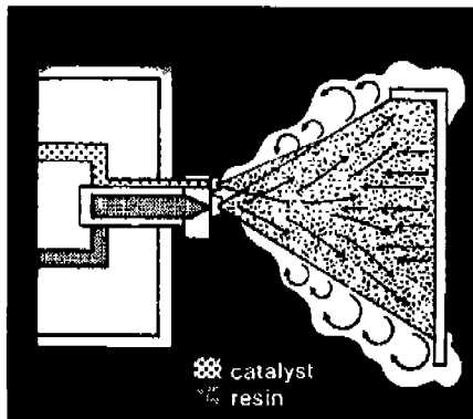
Figure 5-8 Airless Spray Gun Showing Possible Bounce Back from the Mold [Venus-Gusmer]
