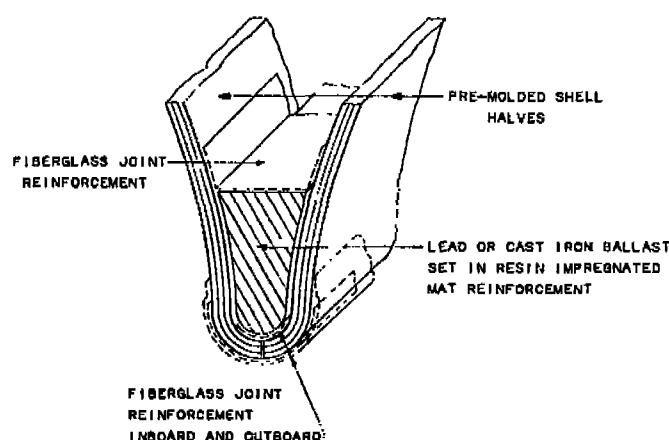
Figure 3-51 Connection of Shell Halves - Cruising Sailboat with Ballast [Gibbs and Cox, Marine Design Manual for FRP ]
