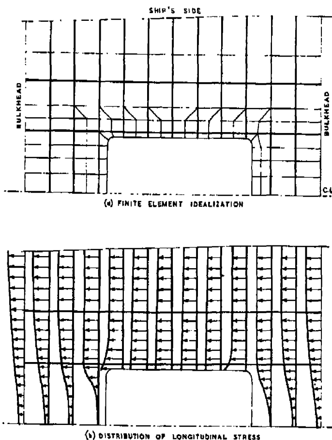
Figure 3-11 Plane Stress Analysis of Hatch Opening [Smith, Buckling Problems in the Design of Fiberglass-Reinforced Plastic Ships ]
