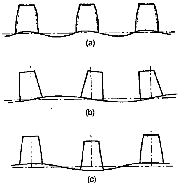
Figure 3-9 Interframe Buckling Modes [Smith, Buckling Problems in the Design of Fiberglass-Reinforced Plastic Ships ]
