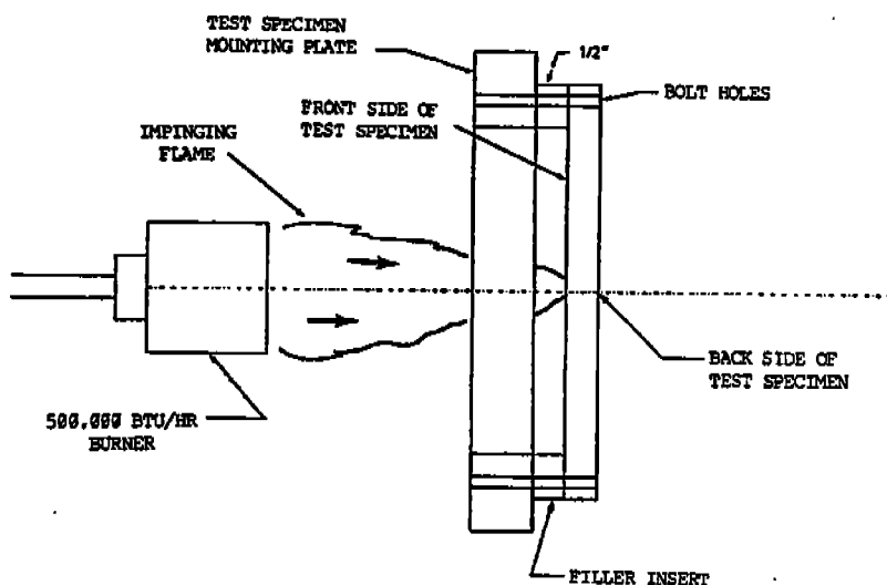
Figure 6-11 Sketch of the DTRC Burn Through Sample and Holder [Rollhauser, Fire Tests of Joiner Bulkhead Panels ]
