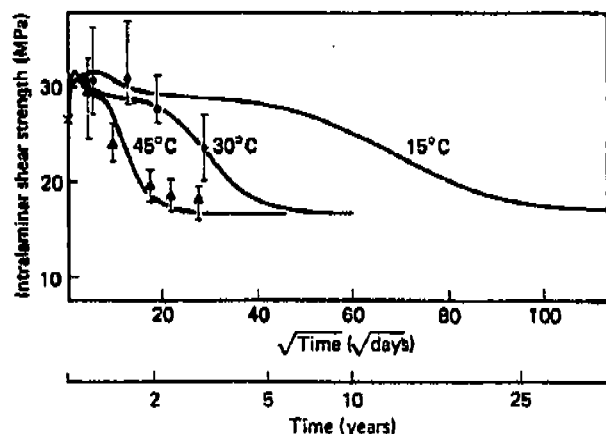
Figure 4-16 Predicted Dry Shear Strength versus Square Root of Immersion Time [Pritchard, The Use of Water Absorbition Kinetic Data to Predict Laminate Property Changes ]
