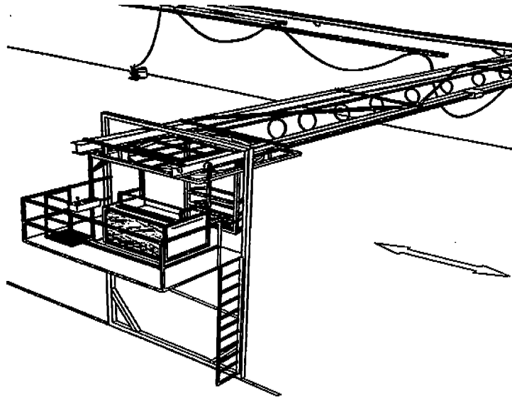
Figure 5-11 Configuration of Semi-Gantry Impregnator [Venus-Gusmer]
