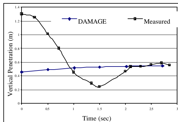
Figure 7: Comparison of Vertical Penetration (ASIS Test No.2)
